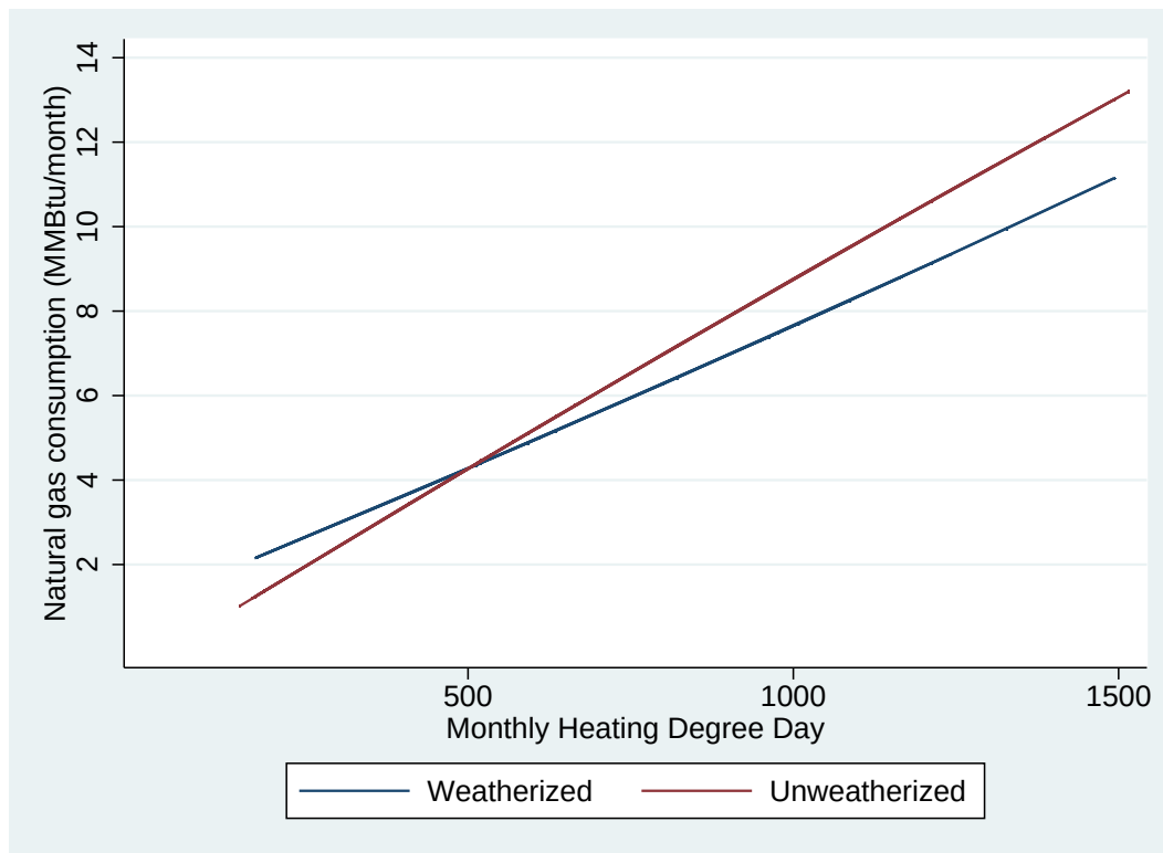
Figure A.2: Building energy performance at weatherized versus unweatherized homes
